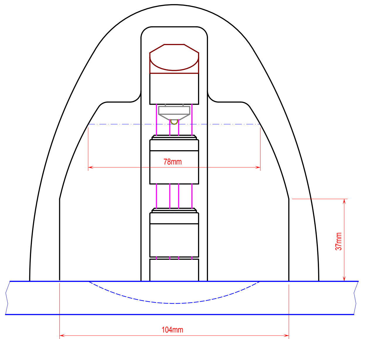
FRONT VIEW
