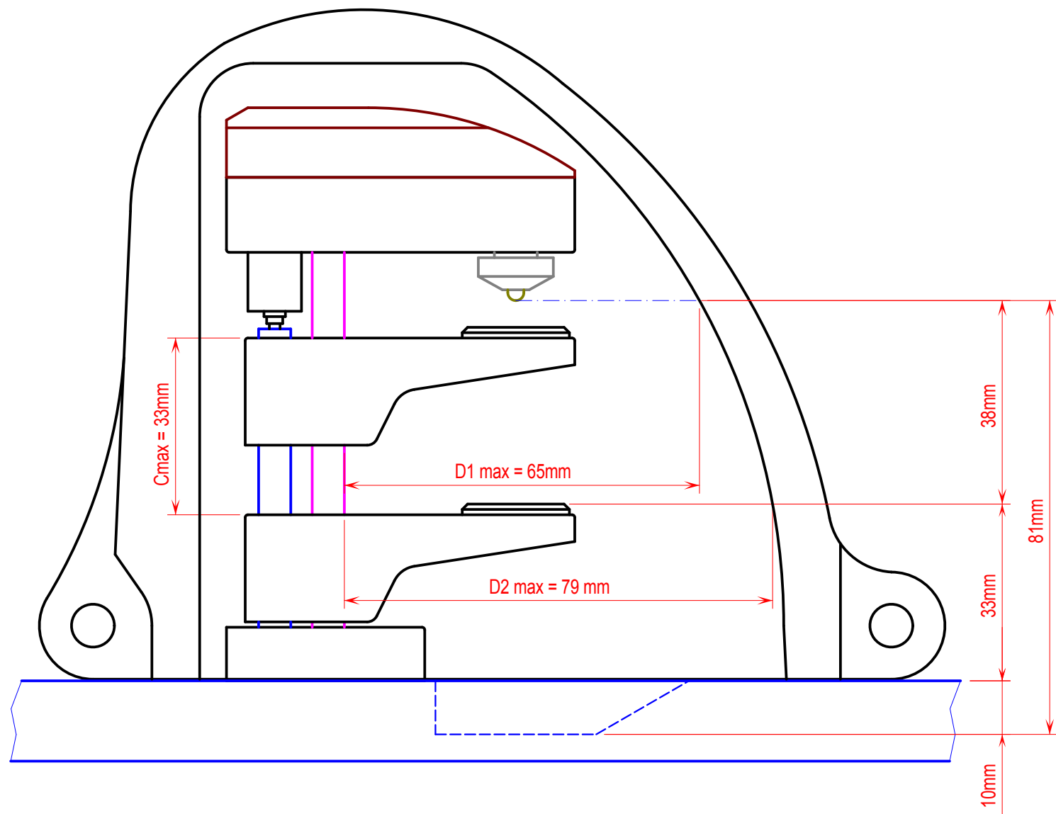
SIDE VIEW
